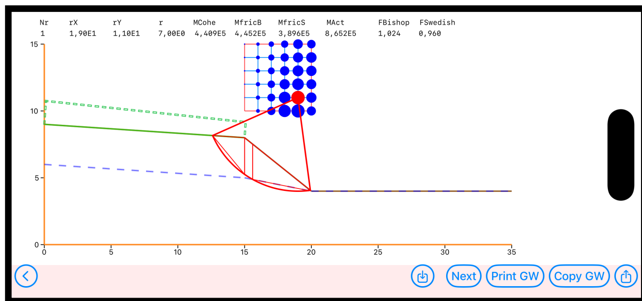
Figure 5: Screen after “Run slope” executed (from file Example 1).
