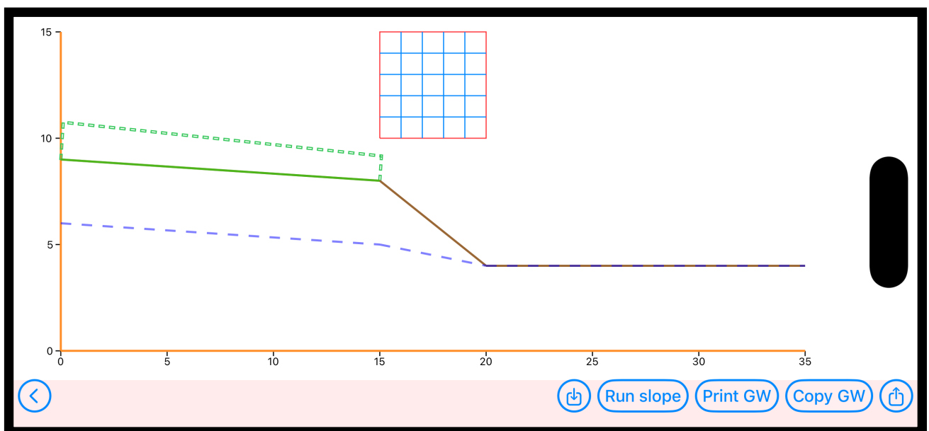
Figure 4: Main action screen (GraphWindow) with action buttons before Run slope is executed (from file Example 1).
