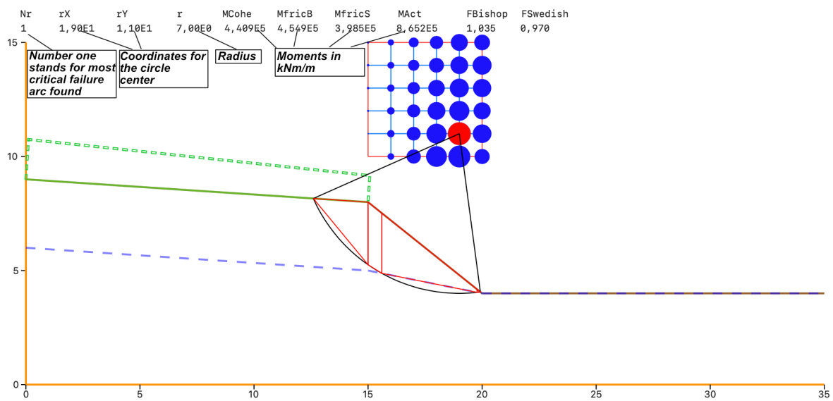
Figure 18: The Graphics display when the Run Slope or Detail command is executed.
