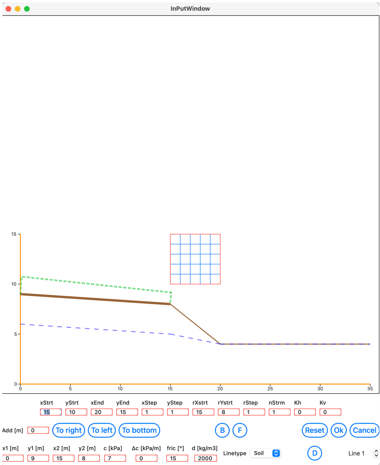
Figure 8: Showing the result of opening the "Example 1.txt" file and then choosing "InputWindow" from the Window menu. 2025 the edit fields and buttons were moved below the graph showing the problem
