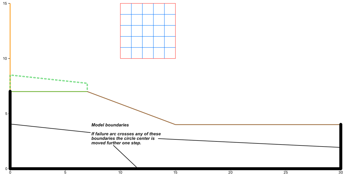
Figure 13: The soil lines defines three boundaries. If a failure arcs crossing with a soil line passes outside any of these boundaries the program will continue with the next slope centre.
