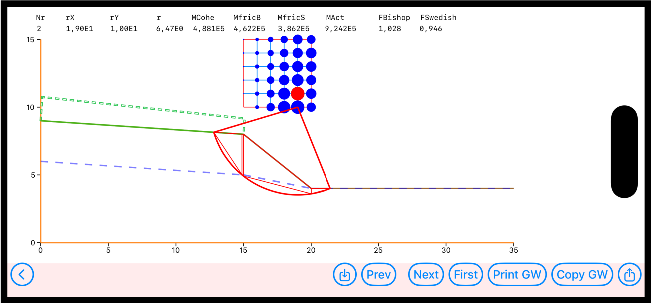
Figure 7: Screen after "Detail" is pressed. Another failure arc than the one with lowest safety factor analysed (from file Example 1)
