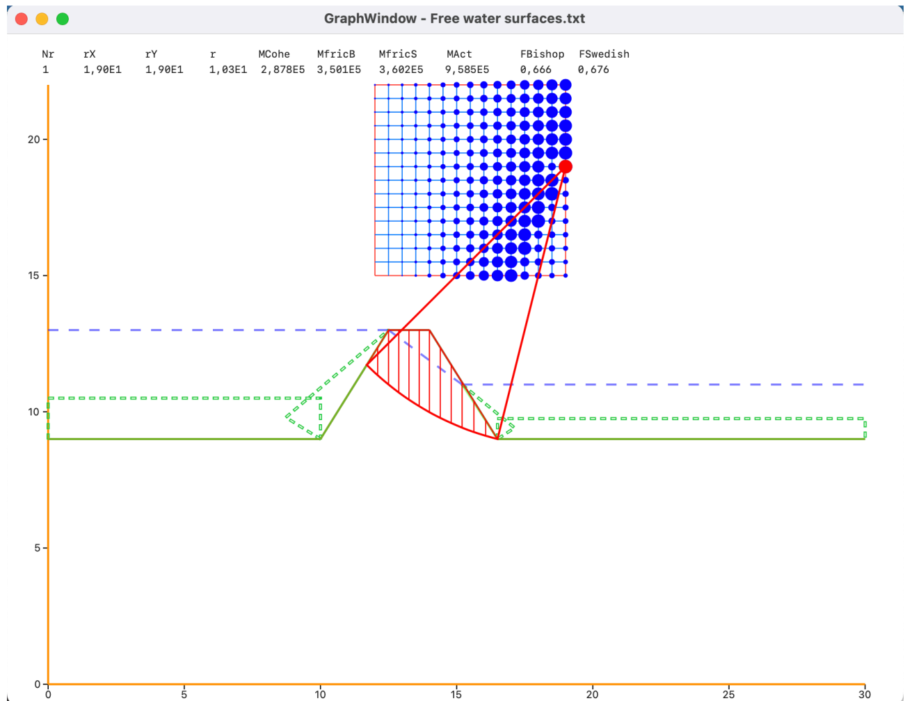
Figure 21: Display of critical center's. The red dot represents the most critical centre found. The bigger dot the more critical centre. The used search square seems to be a little bit to much to the left and probably a bit low.
