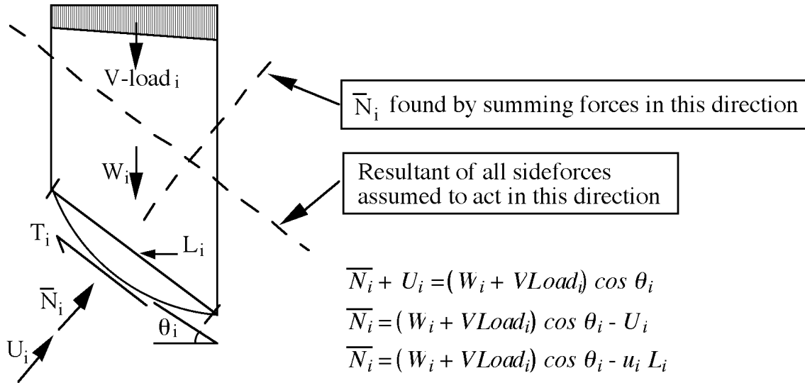
Figure 15: Forces considered in the Swedish method of slices.
