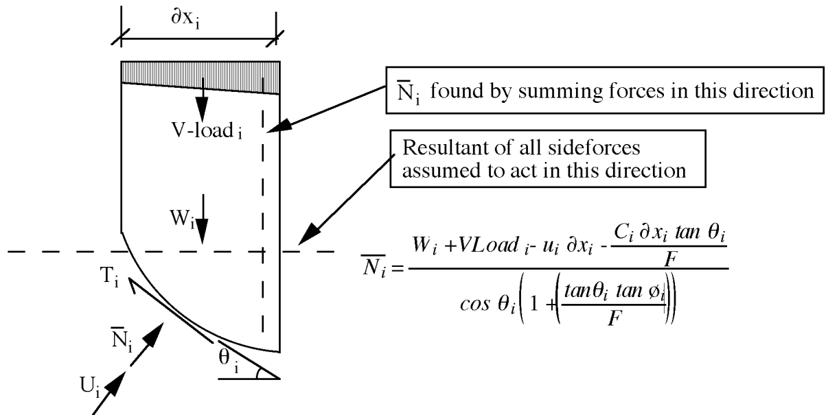
Figure 16: Forces considered in simplified Bishop's method of slices.
