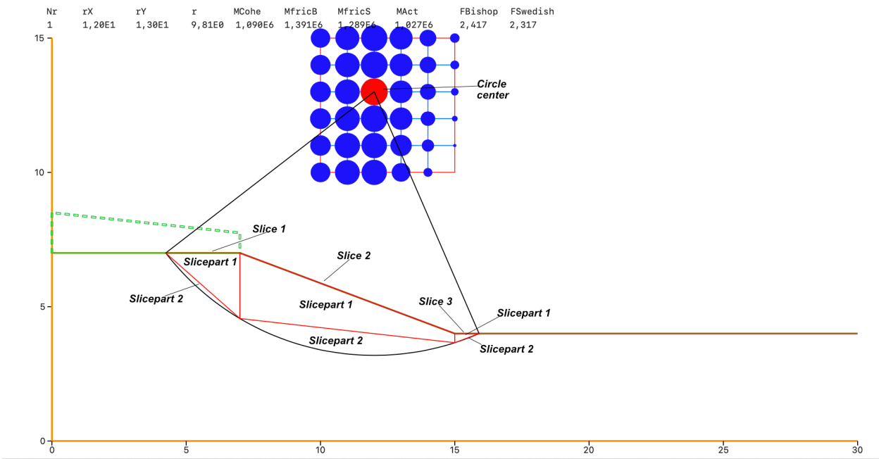
Figure 14: The program first divides the slope into vertical slices then divides each slice into parts separated by soil lines and for the last part, the intersected failure arc.
