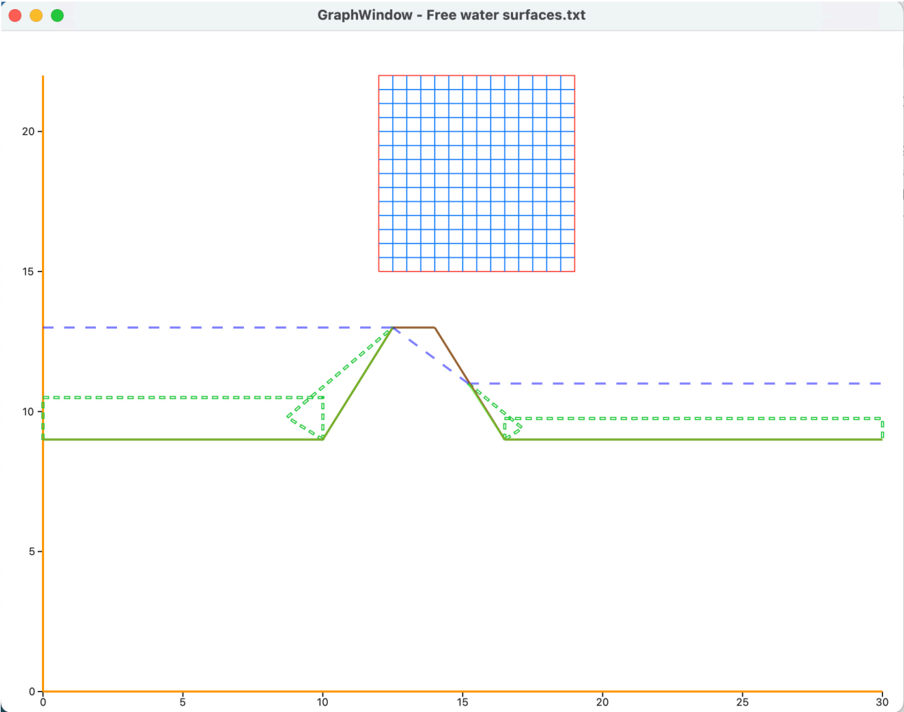
Figure 20: Example of how to deal with free water surfaces.
