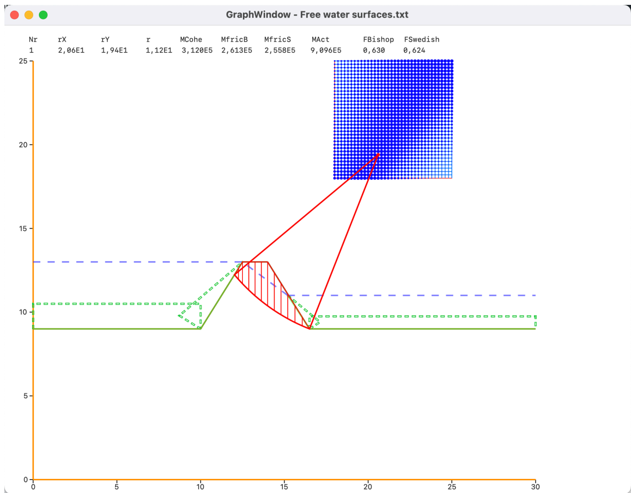
Figure 22: Display of critical center's. Second try. Seems to be OK.
