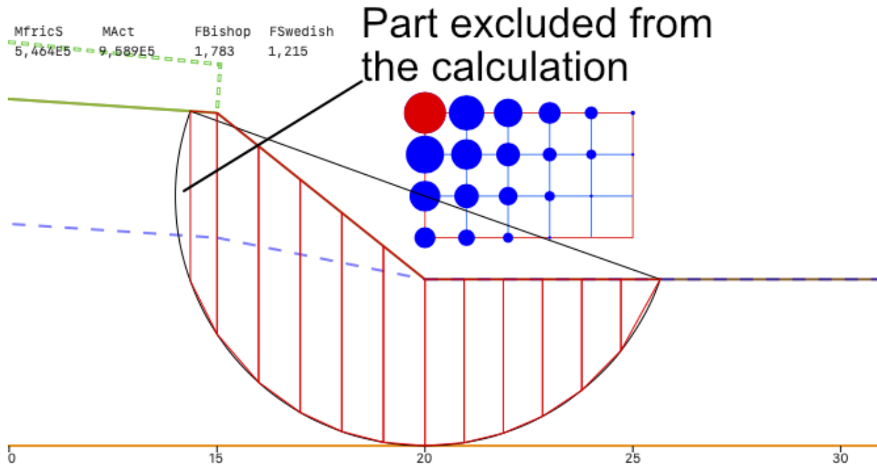
Figure 17: Arc centre under the start point of the failure arc (from file “Bad search example”).
